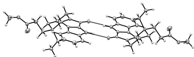
Figure 2. X-ray structure of (±)-leucomidine B ( 2 ).
