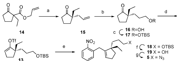
Scheme 2. Synthesis of cyclopentene 5 . a) [\text{Pd}(\text{dba})_3] (2.5 mol%), ( S )- t BuPHOX (6.25 mol%), THF ( c 0.067 M), 25 °C, 3 h, 87% yield, 86% ee ; b) disiamyl borane (2.5 equiv), THF, 0 °C to RT, 2 h then \text{H}_2\text{O}_2/\text{NaOH} , RT, 1 h; c) TBSCl (1.2 equiv), imidazole (1.5 equiv), DMF, RT, 12 h, 85% over 2 steps; d) LiHMDS (1.1 equiv), THF, –78 °C, 45 min then \text{PhNTf}_2 (1.2 equiv), –78 °C to RT, 12 h, 92%; e) potassium 2-(2-nitrophenyl)acetate ( 12 , 2.5 equiv), [\{\text{Pd}(\text{allyl})\text{Cl}\}_2] (5 mol%), XPhos (15 mol%), diglyme, 140 °C, 2 h, 52%; f) \text{AcCl} (0.20 equiv), MeOH, RT, 1 h; g) \text{MsCl} (1.2 equiv), \text{Et}_3\text{N} (1.5 equiv), DMF, RT, 5 h then \text{NaN}_3 (3.0 equiv), RT, 12 h, 84% over 2 steps. dba = 1,5-diphenyl-1,4-pentadien-3-one, THF = tetrahydrofuran, TBS = tert -butyldimethylsilyl, DMF = N,N -dimethylformamide, LiHMDS = lithium hexamethyldisilazide, Tf = triflate.
